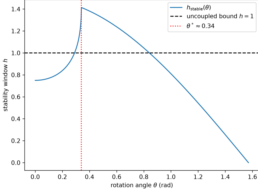
Figure 1: Stability window h_{\text{stable}}(\theta) for the rotated two-block field R(\theta)A\tilde{R}(\theta) with A = \text{diag}(-1, -2) . The dashed line marks the uncoupled bound h = 1 ; the dotted vertical line marks the angle of maximum stability \theta^* = \arccos(2\sqrt{2}/3) \approx 0.3398 , where h_{\text{stable}} = \sqrt{2} . The window is non-monotonic: it grows from the uncoupled bound at \theta = 0 to its peak at \theta^* , then decreases continuously to zero at the permutation limit \theta = \pi/2 .
