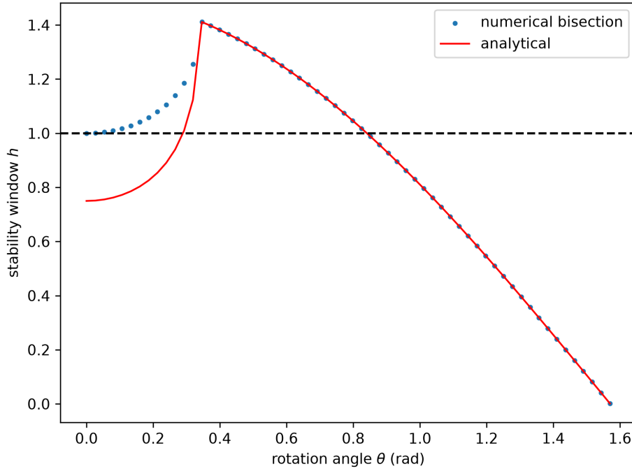
Figure 3: Verification scatter: the analytical stability window h_{\text{stable}}(\theta) from equation (??) (red curve) against the boundary located by direct numerical bisection on the spectral radius \rho(I + hR(\theta)A\hat{R}(\theta)) = 1 (blue dots). The dashed horizontal line marks the uncoupled bound h = 1 . The two agree to numerical precision across the full range 0 \leq \theta < \pi/2 .
