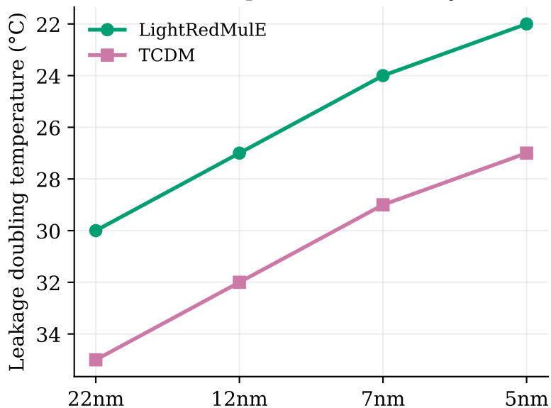
(b) Temperature sensitivity
