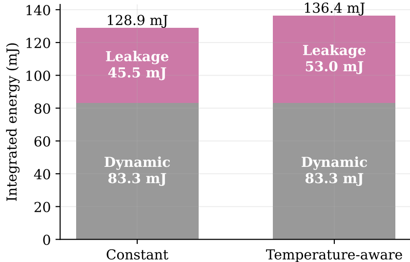
(b) Energy over the full application
