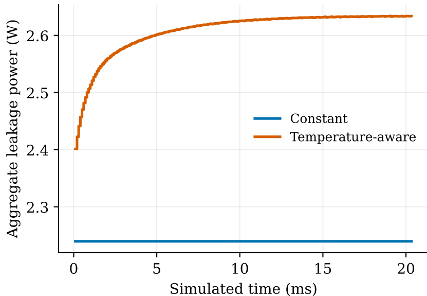
(a) Chip-level modeled leakage
