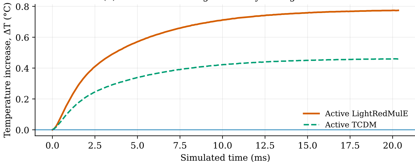
(b) Additional heating caused by leakage feedback
