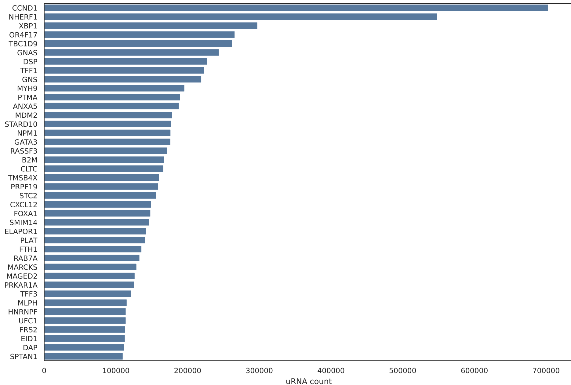
Top genes by high-quality unassigned RNA count
