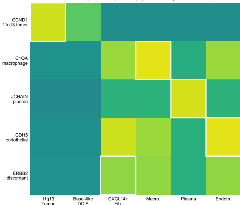
f uRNA-only COSTE proximity (1 - SSS; higher is closer)
