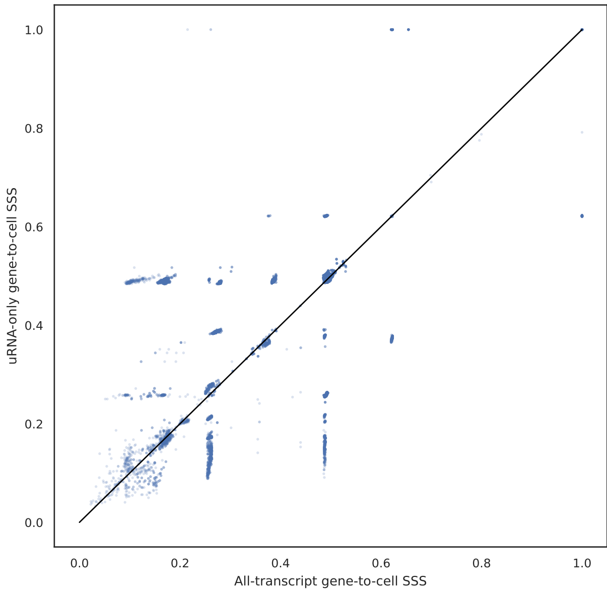
All-transcript vs uRNA-only SSS (Spearman 0.652)
