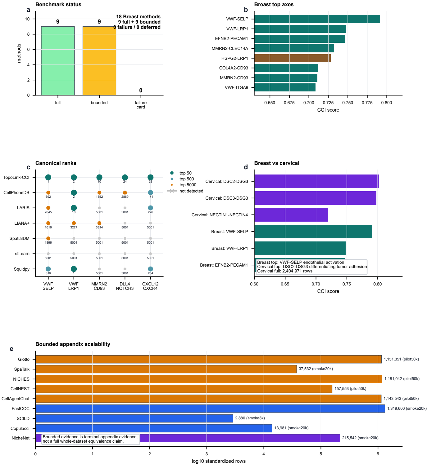
Figure 2 | Whole-dataset benchmarking and biological interpretation
