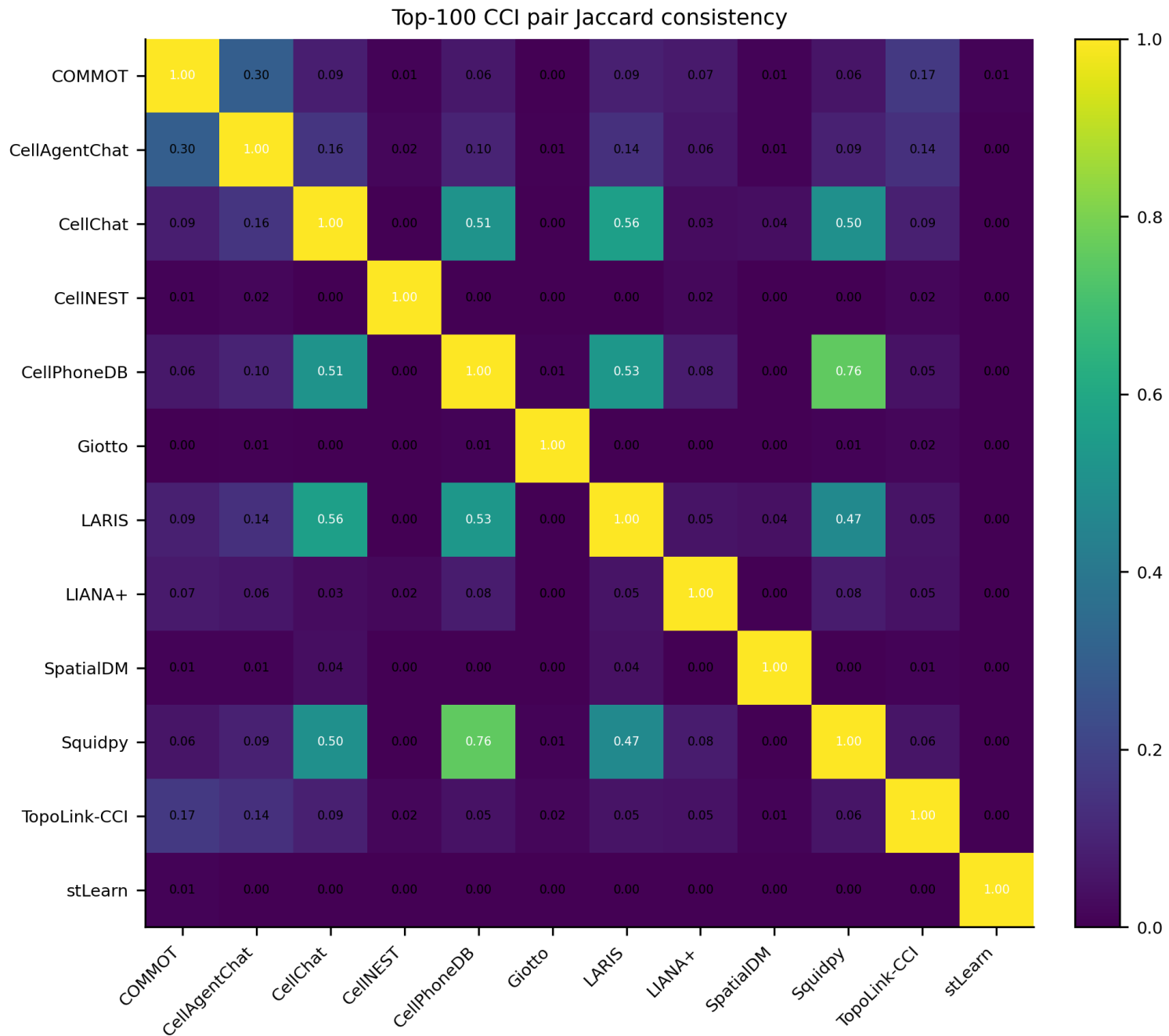
Figure panel 6. Top-100 pair Jaccard consistency
