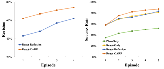
Fig. 5. Result of revision and success rate with different episodes. CARF effectively improves the performance of long-term tasks.
