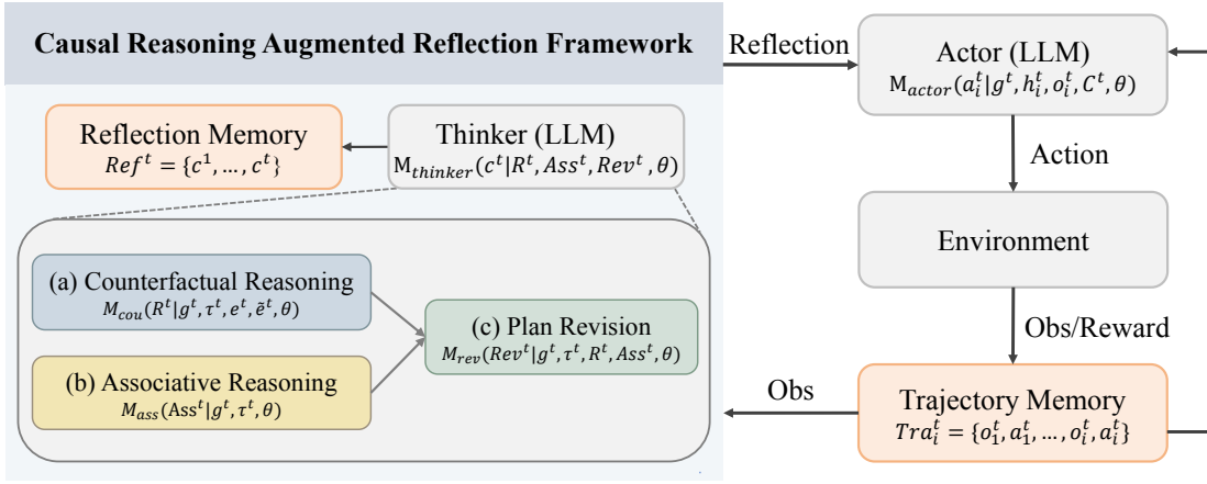
Fig. 2. The framework of CARF. Our framework operates by taking historical task information and environmental feedback as input and producing reflection results as output. The framework comprises three stages: 1. Counterfactual Reasoning is responsible for identifying and correcting critical erroneous steps and analyzing the RCE. 2. Associative Reasoning is tasked with inferring about the associations. 3. Plan Revision is charged with generating the action plan revisions for subsequent trials. Additionally, we have introduced a Memory Management module to manage the historical results generated.
