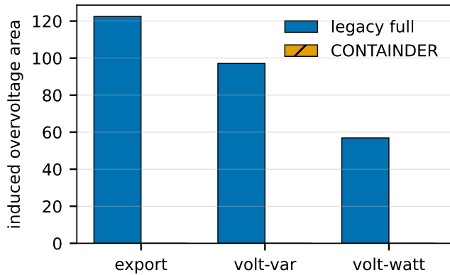
Fig. 5. Induced overvoltage area by attack family (IEEE 8500, light load). Narrowing scope contains overvoltage driven by active or reactive authority.
