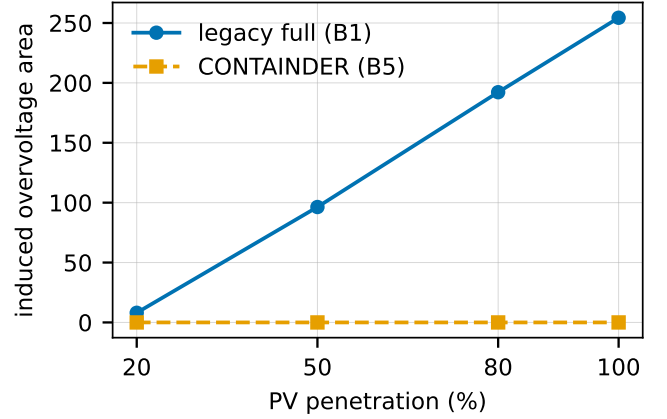
Fig. 4. Induced overvoltage area versus PV penetration (IEEE 8500, light load, 5 seeds). Harm scales with penetration under the legacy baseline; containment is penetration-independent under CONTAINER.
