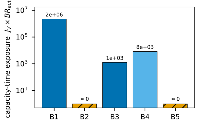
Fig. 3. Capacity-time exposure by baseline on the IEEE 8500-node feeder (light load, log scale). Persistence multiplies exposure only at full scope (B1 vs B3); at narrow scope (B2, B5) it is inert, the persistence–scope interaction. Bars floored at 1 for log display; B2, B5, B6 are \approx 0 .
