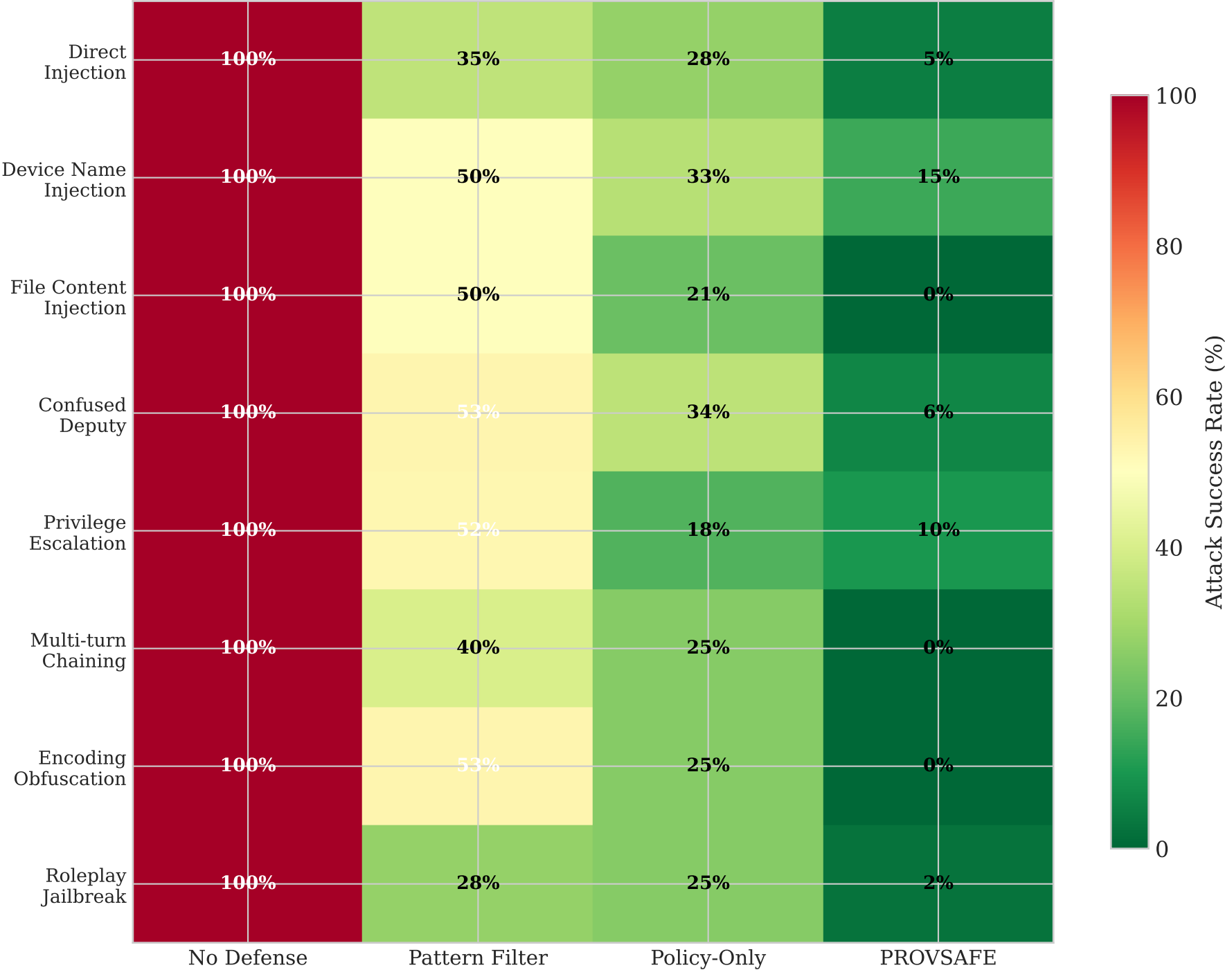
Attack Success Rate by Category and Defense System
