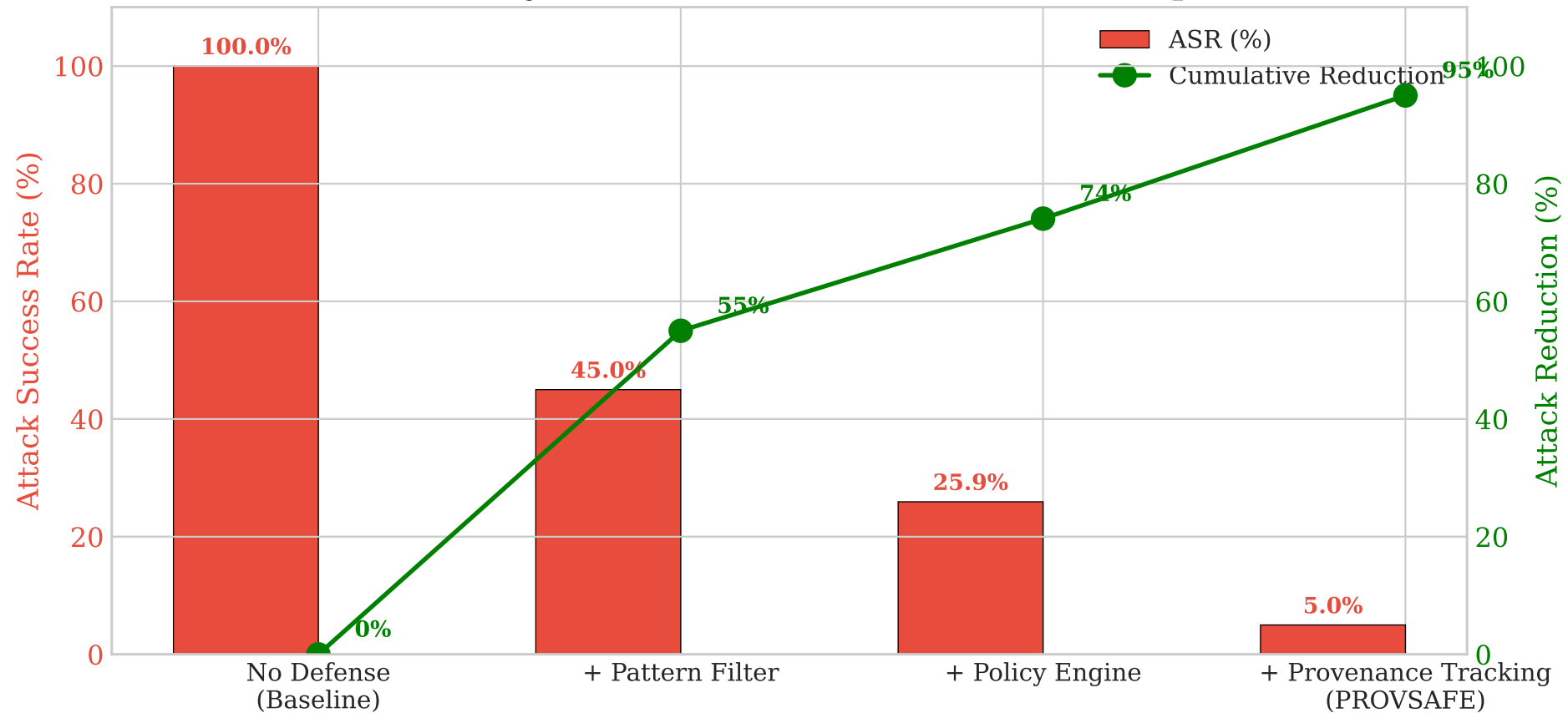
Ablation Study: Contribution of Each Defense Component
