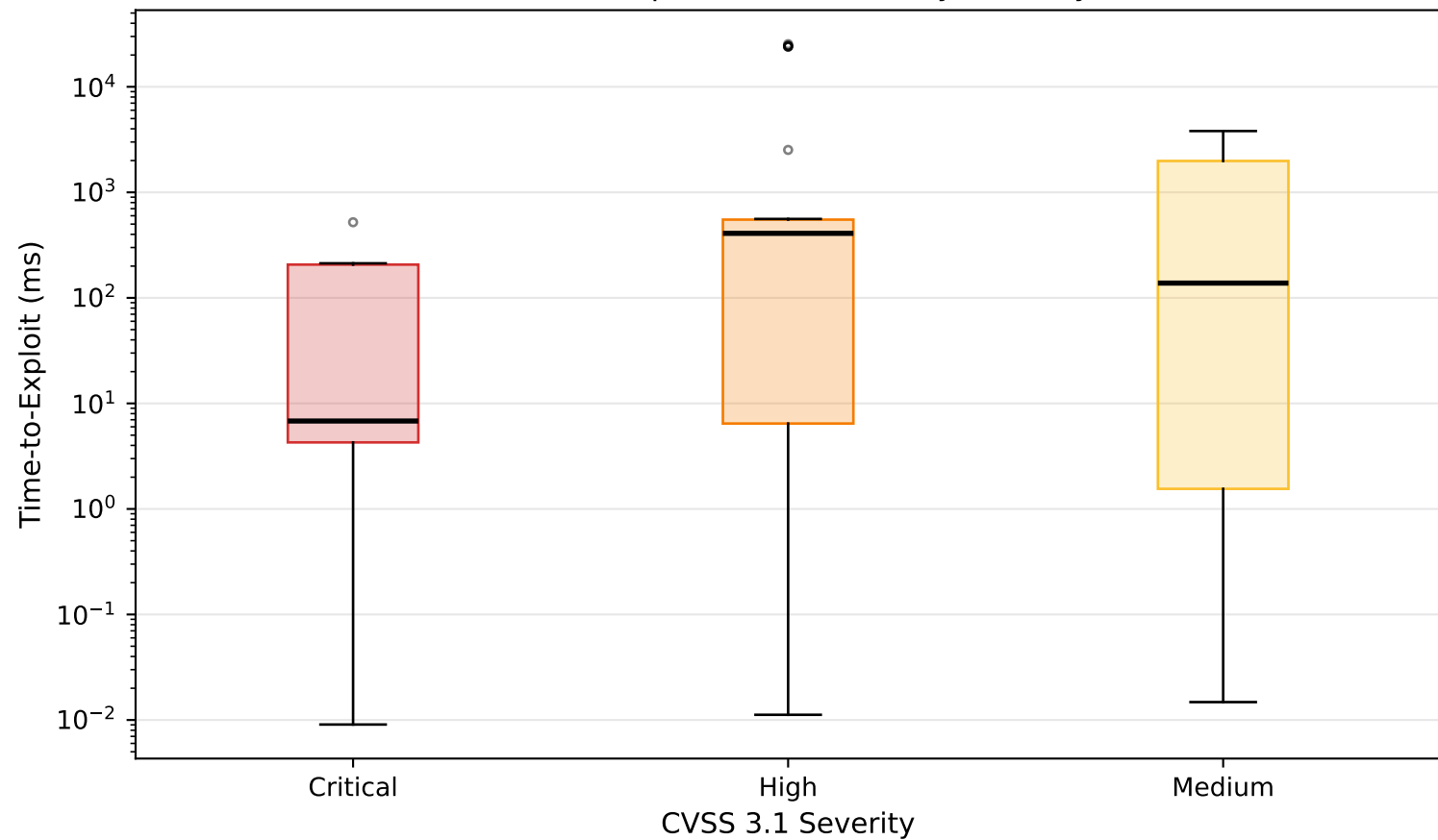
Time-to-Exploit Distribution by Severity
