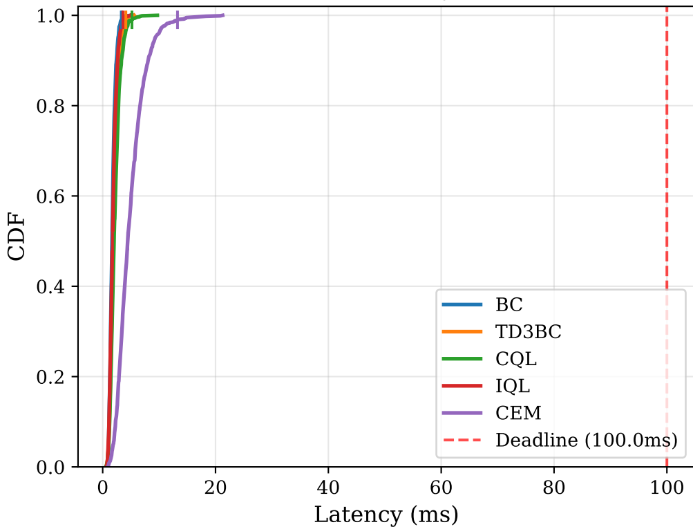
Decision Latency CDF
