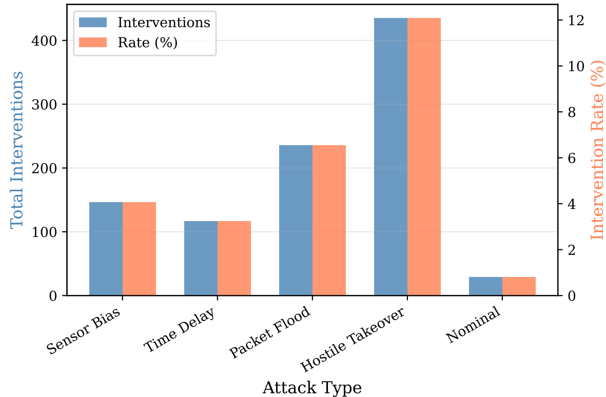
Interventions by Attack Type
