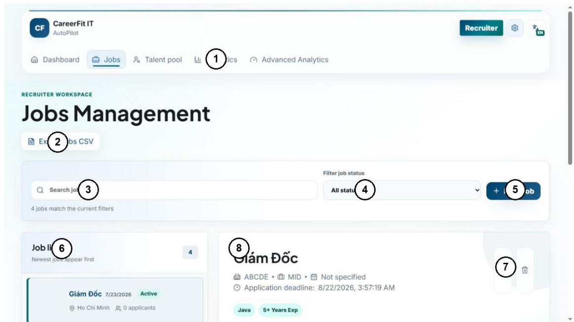
Figure 3.17. Annotated interface for Job and applicant management
