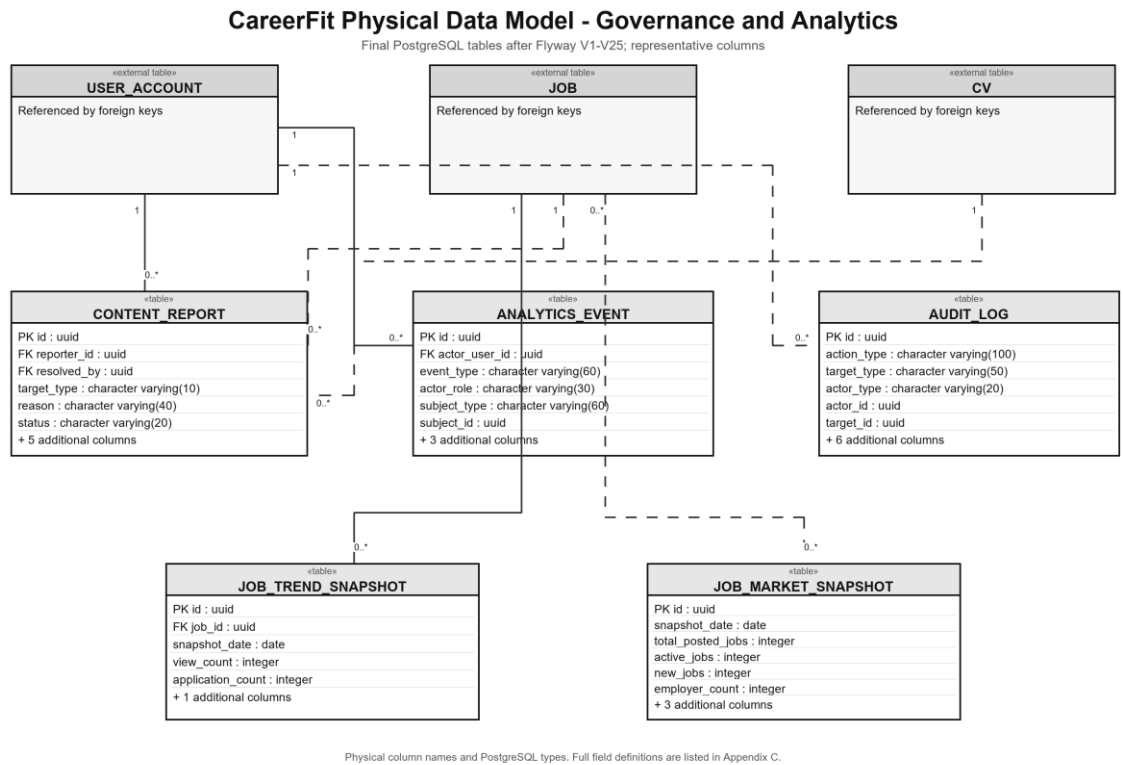
Figure 3.10. CareerFit physical data model - governance and analytics tables
