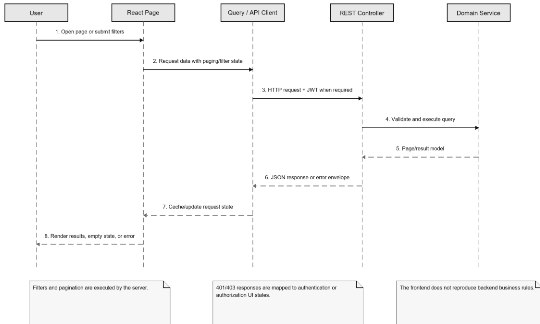
Figure 3.34. Frontend request and API-response sequence
