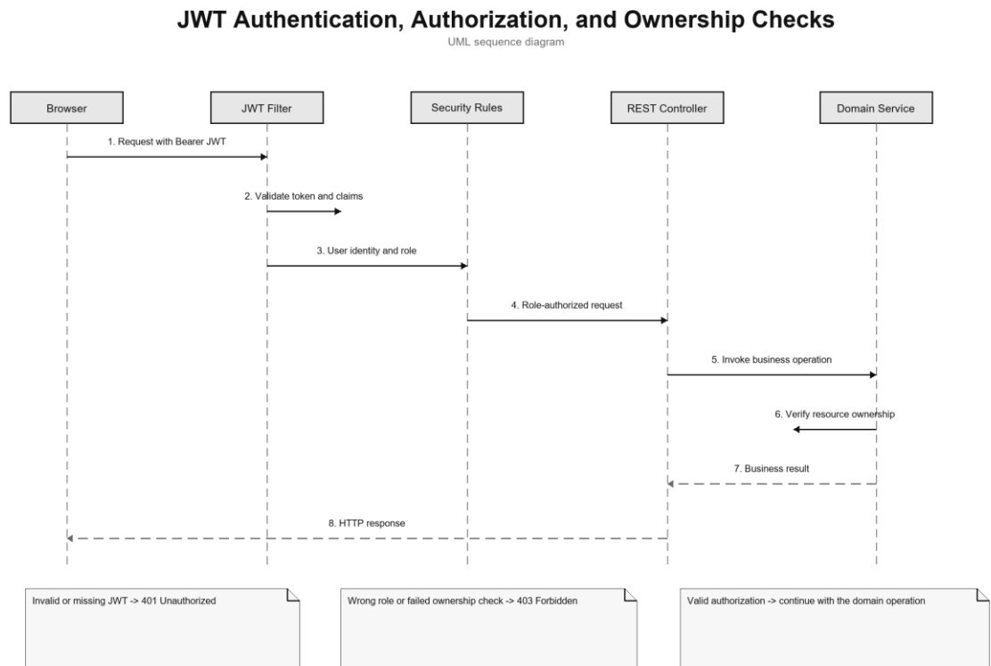
Figure 3.13. JWT authentication, role authorization, and ownership-check sequence
