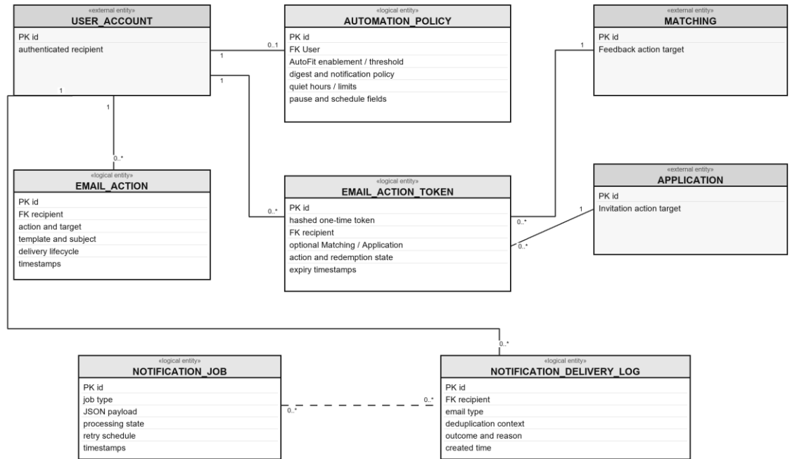
Figure 3.5. CareerFit logical data model - automation and communication
