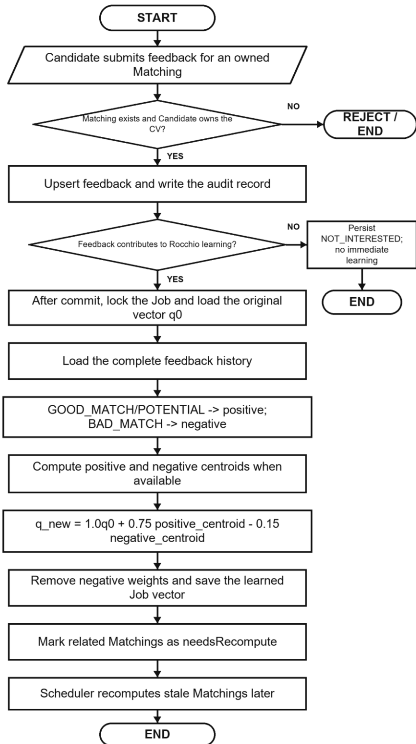
Figure 3.17. Rocchio feedback-learning and recomputation flowchart
