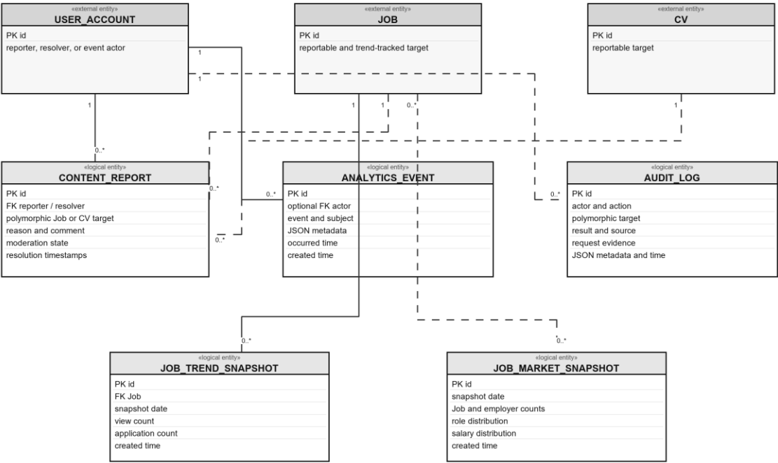
Figure 3.6. CareerFit logical data model - governance and analytics
