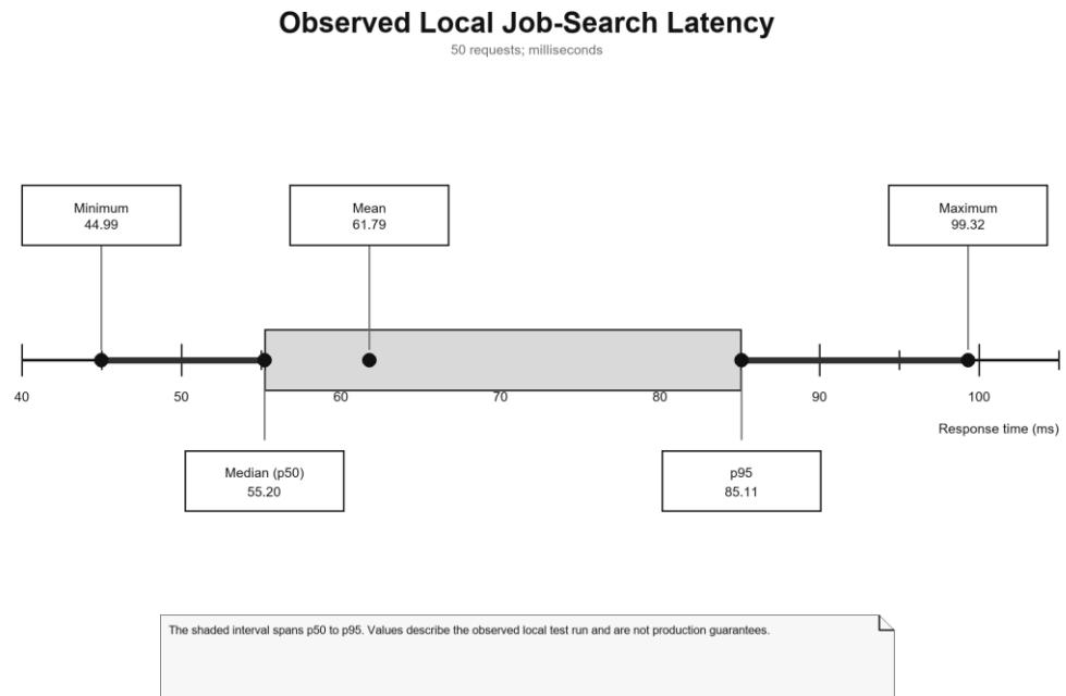
Figure 4.2. Observed local Job-search latency statistics
