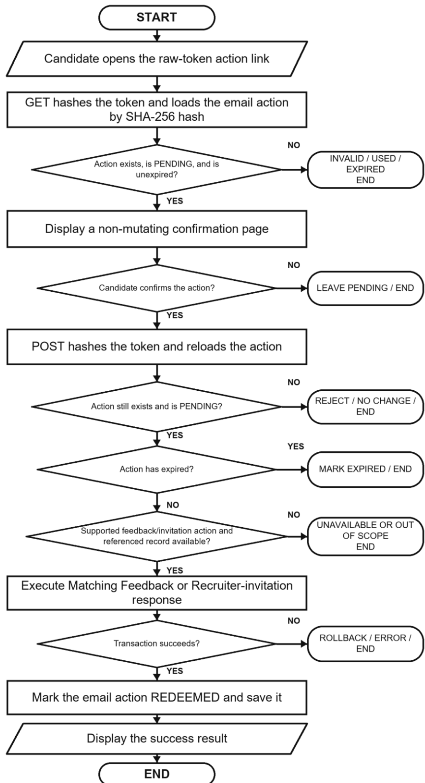
Figure 3.21. Actionable-email confirmation and redemption flowchart
