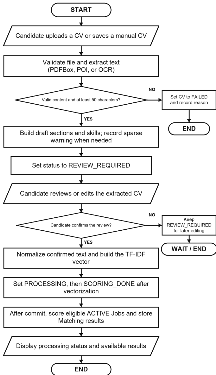
Figure 3.14. CV ingestion, review, confirmation, and matching flowchart
