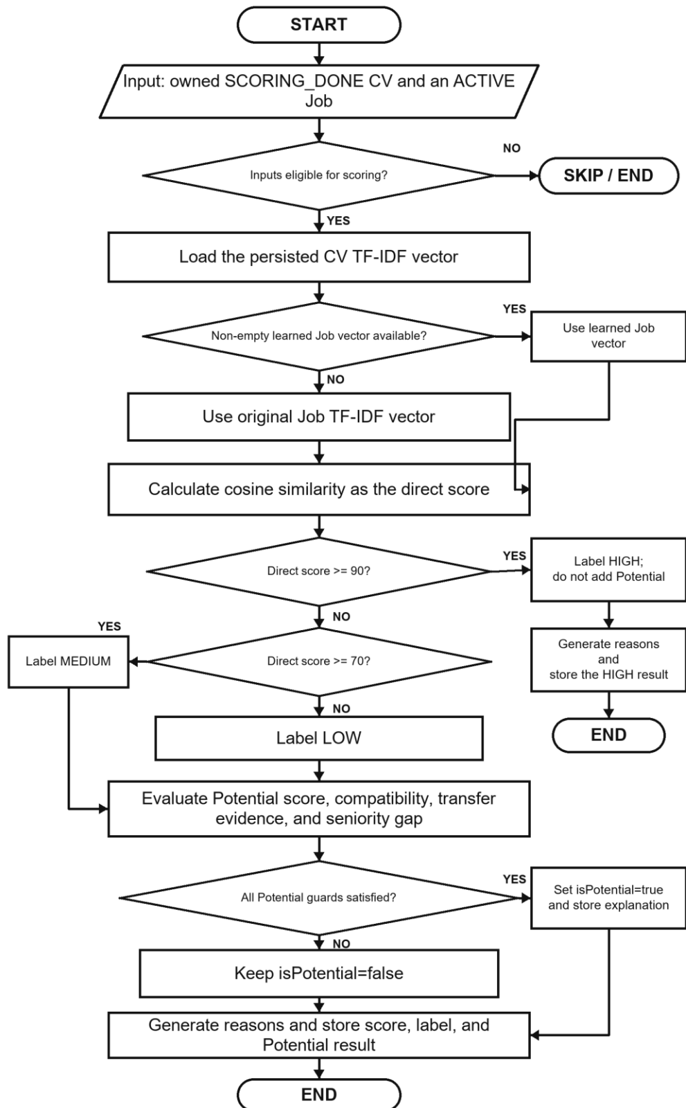
Figure 3.16. CV-Job matching and Potential assessment flowchart
