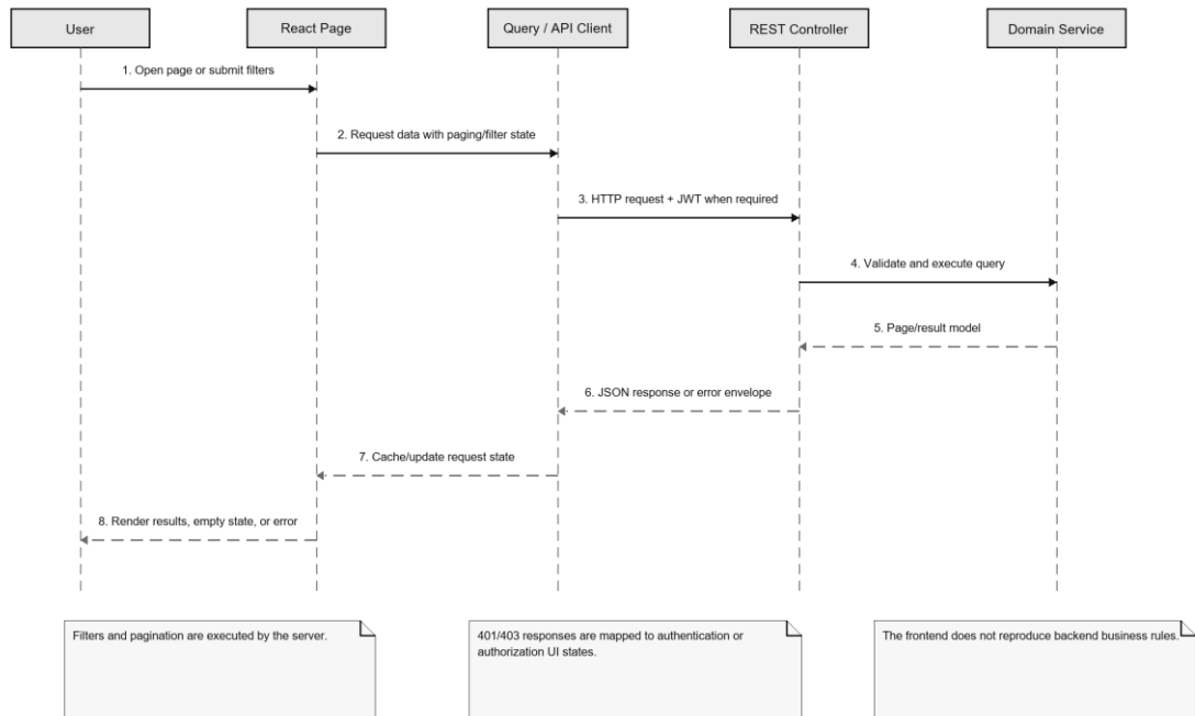
Figure 3.22. Frontend request and API-response sequence
