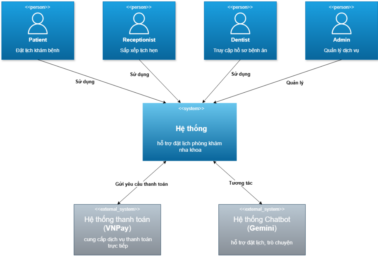
Figure 1. Context Diagram
