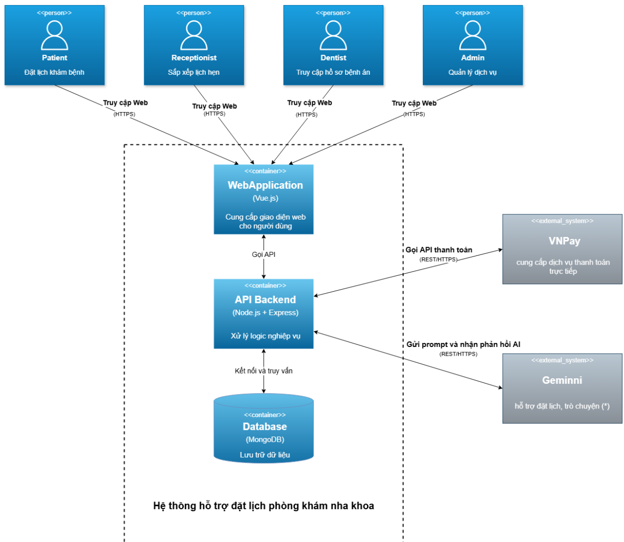
Figure 2. Container Diagram
