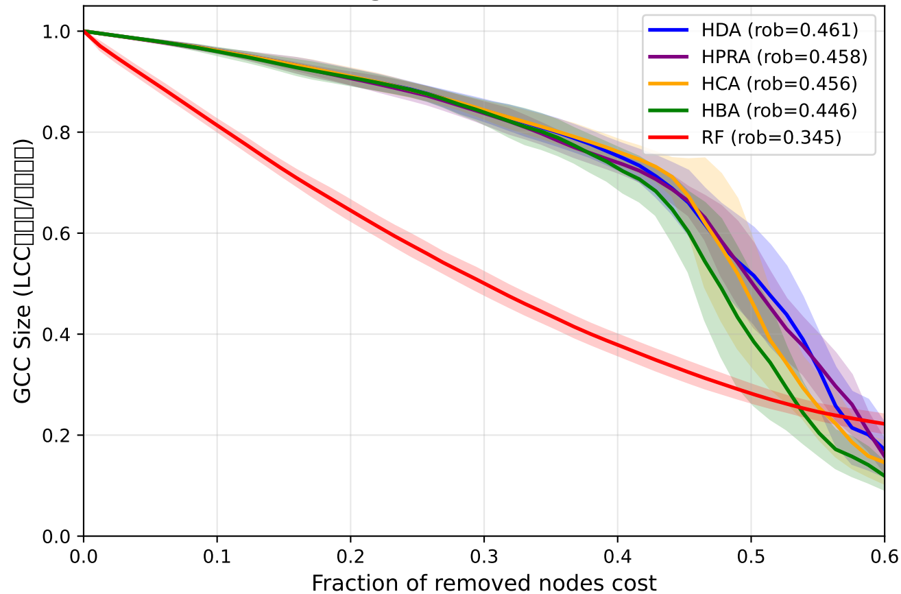
Network Dismantling: GCC Size vs Removed Nodes Cost
