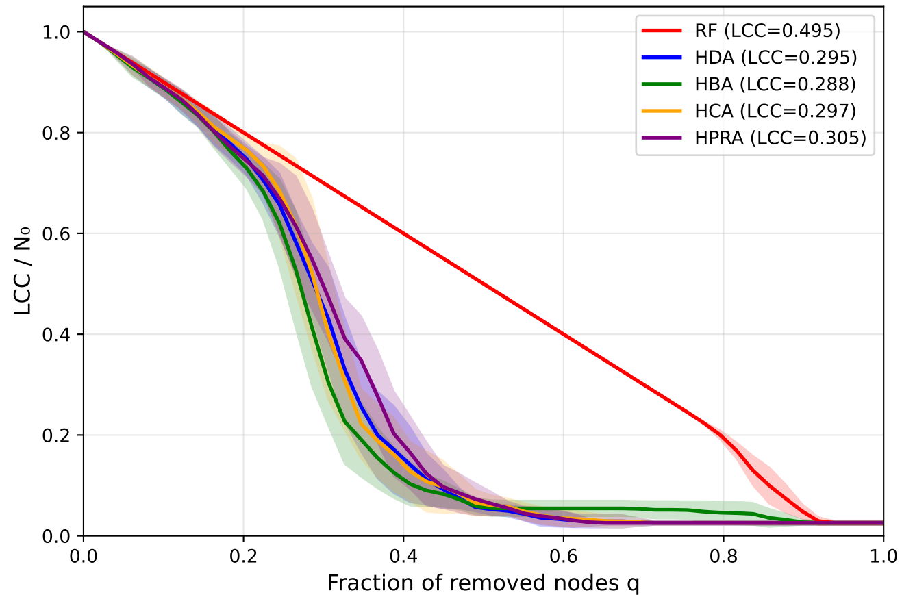
LCC vs Fraction of Removed Nodes
