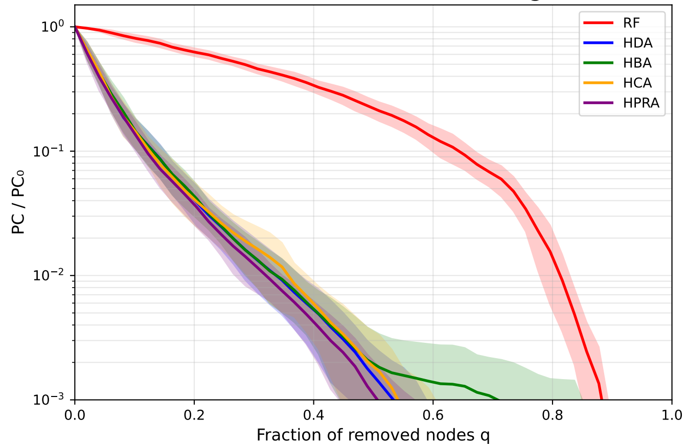
PC vs Fraction of Removed Nodes (log scale)
