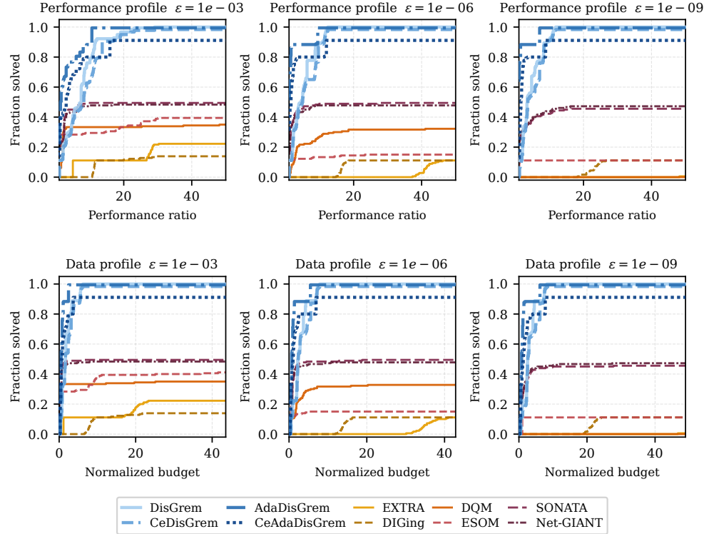
Fig. 1: Iteration-budget profiles at three precision levels \varepsilon \in \{10^{-3}, 10^{-6}, 10^{-9}\} . Top: performance profiles; bottom: data profiles. A solver’s curve at ordinate \pi indicates it solves a \pi -fraction of the problem–MC instances within the given budget.
