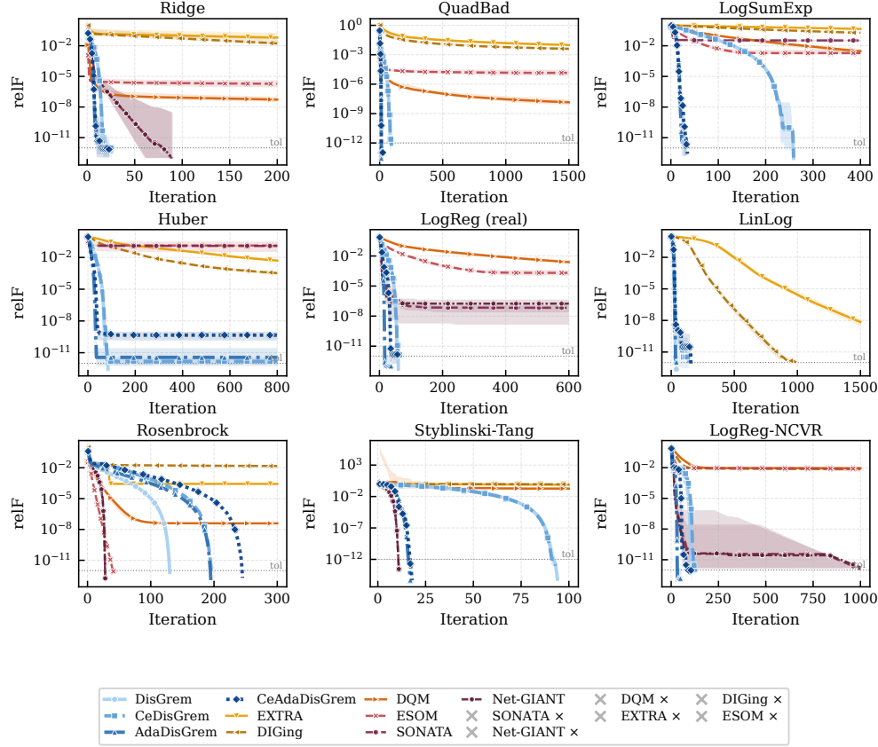
Fig. 3: relF vs. iteration on all nine test functions ( N=10, 20 MC runs; synthetic objectives use d=30 , whereas the two logistic-regression objectives use the d=22 SVMGUIDE3 feature dimension; logarithmic communication implementation). Solid curves: DISGREM family; dashed: baselines. Shaded bands: interquartile range. Legend entries marked by \times indicate algorithms whose median curve is not drawn because the corresponding runs terminated by NaN, overflow, or divergence.
