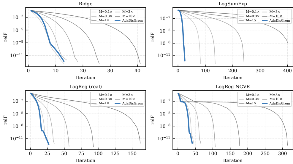
Fig. 6: ADADISGREM (bold blue) vs. DISGREM at five fixed- M values ( 0.1\times – 10\times the baseline M^* ; gray curves light-to-dark). The adaptive variant is competitive with the best fixed choice on most functions and avoids failures at aggressive fixed- M choices.
