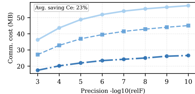
Huber
