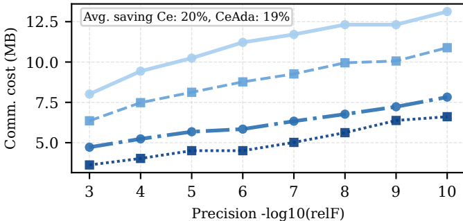
Huber
