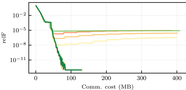
Huber
