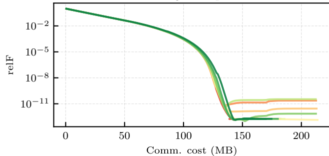
LogSumExp
