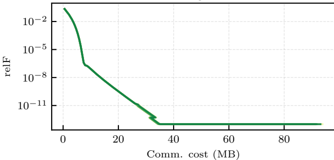
Ridge
