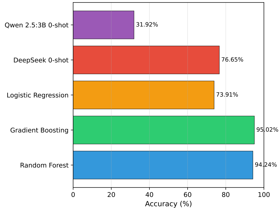
Test Set Accuracy Comparison
