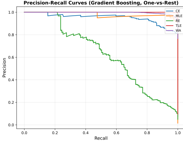
Fig. 6. Precision-Recall curves for Gradient Boosting (One-vs-Rest, test set n = 2,672 )
