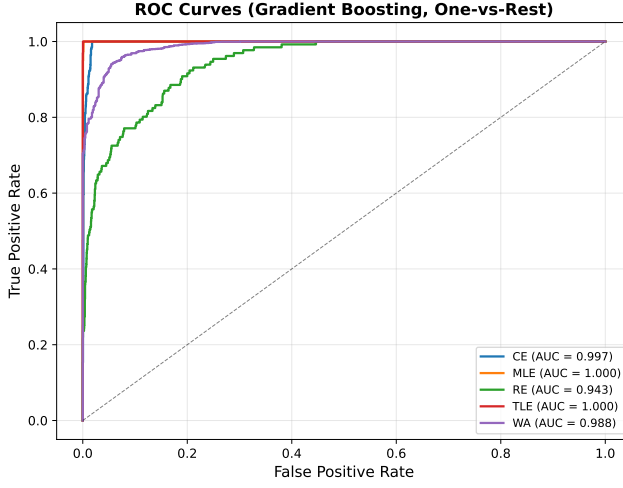
Fig. 5. ROC curves for Gradient Boosting (One-vs-Rest, test set n = 2,672 ). AUC values: CE = 0.997, MLE = 1.000, TLE = 1.000, WA = 0.988, RE = 0.943
