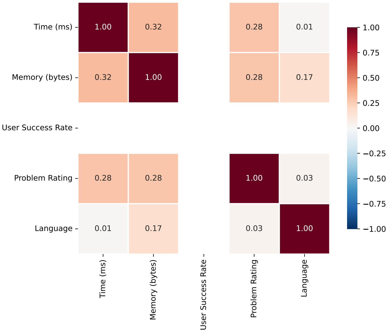
Feature Correlation Matrix (n=14,673)
