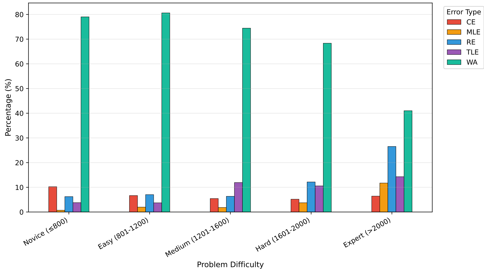
Error Type Distribution Across Difficulty Levels (n=14,673)
