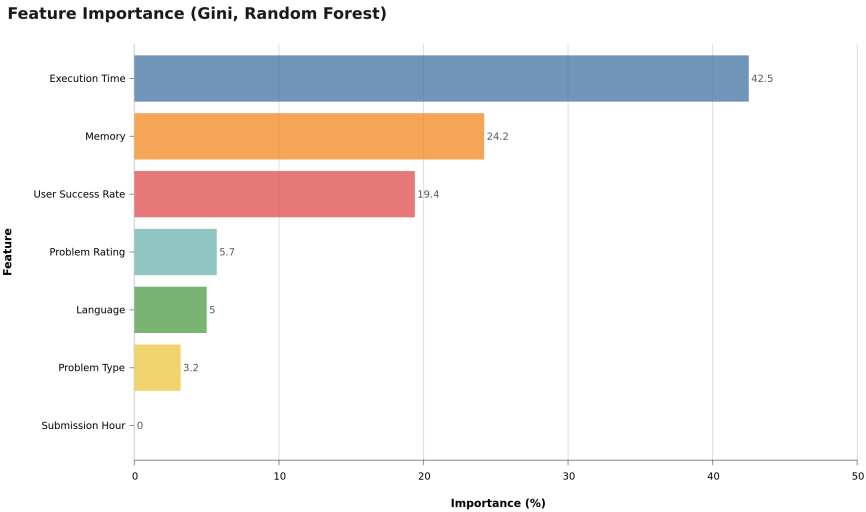
Fig. 4. Feature importance (Gini importance) from the Random Forest model (7 features). Execution time ( time_consumed_ms ) shows the highest importance (42.5%), followed by memory consumption (24.2%), user success rate (19.4%), problem difficulty (5.7%), programming language (5.0%), problem type (3.2%), and submission hour (0.0%).
