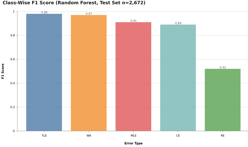
Fig. 3. Class-wise F1 scores (Random Forest, test set n = 2672 ). Four error types—Compilation Error, Memory Limit Exceeded, Time Limit Exceeded, and Wrong Answer—achieve strong F1 ( \geq 0.89 ), whereas Runtime Error (RE) is markedly weaker ( F1 = 0.52 ). This asymmetry reflects the platform-encoding boundary : CE/TLE/MLE are cleanly separable by execution time and memory, while RE submissions share no distinctive metadata signature.
