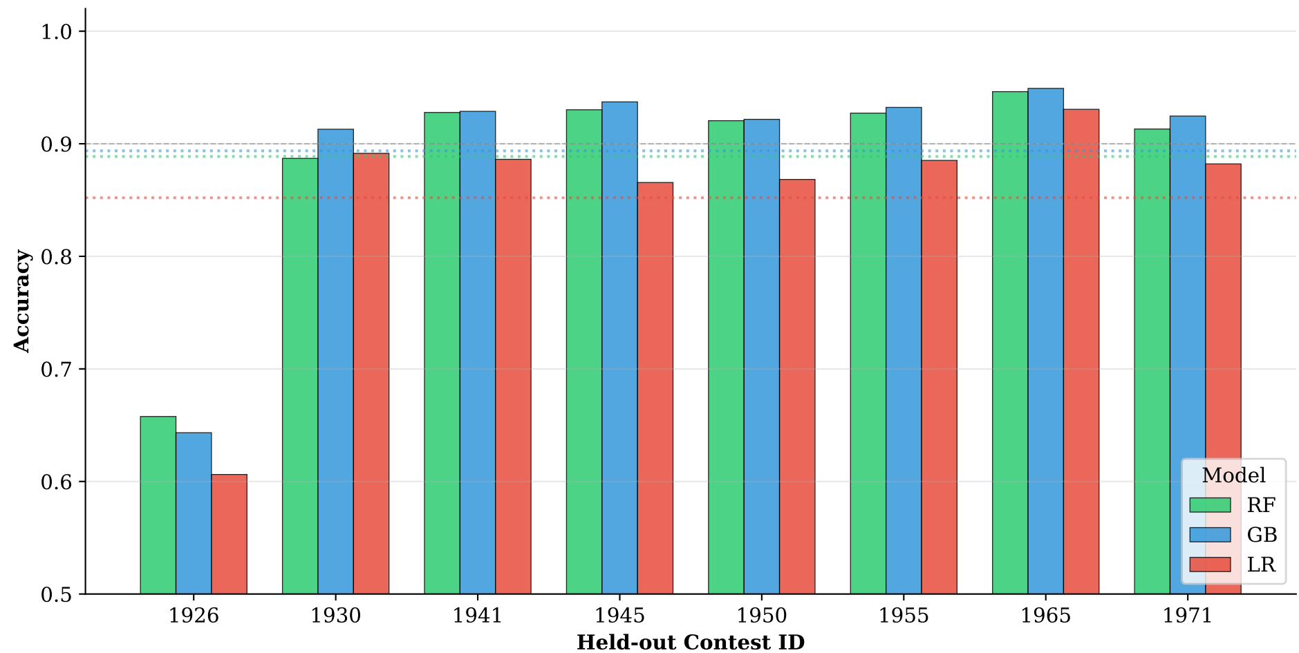
Leave-One-Contest-Out Cross-Validation Results
