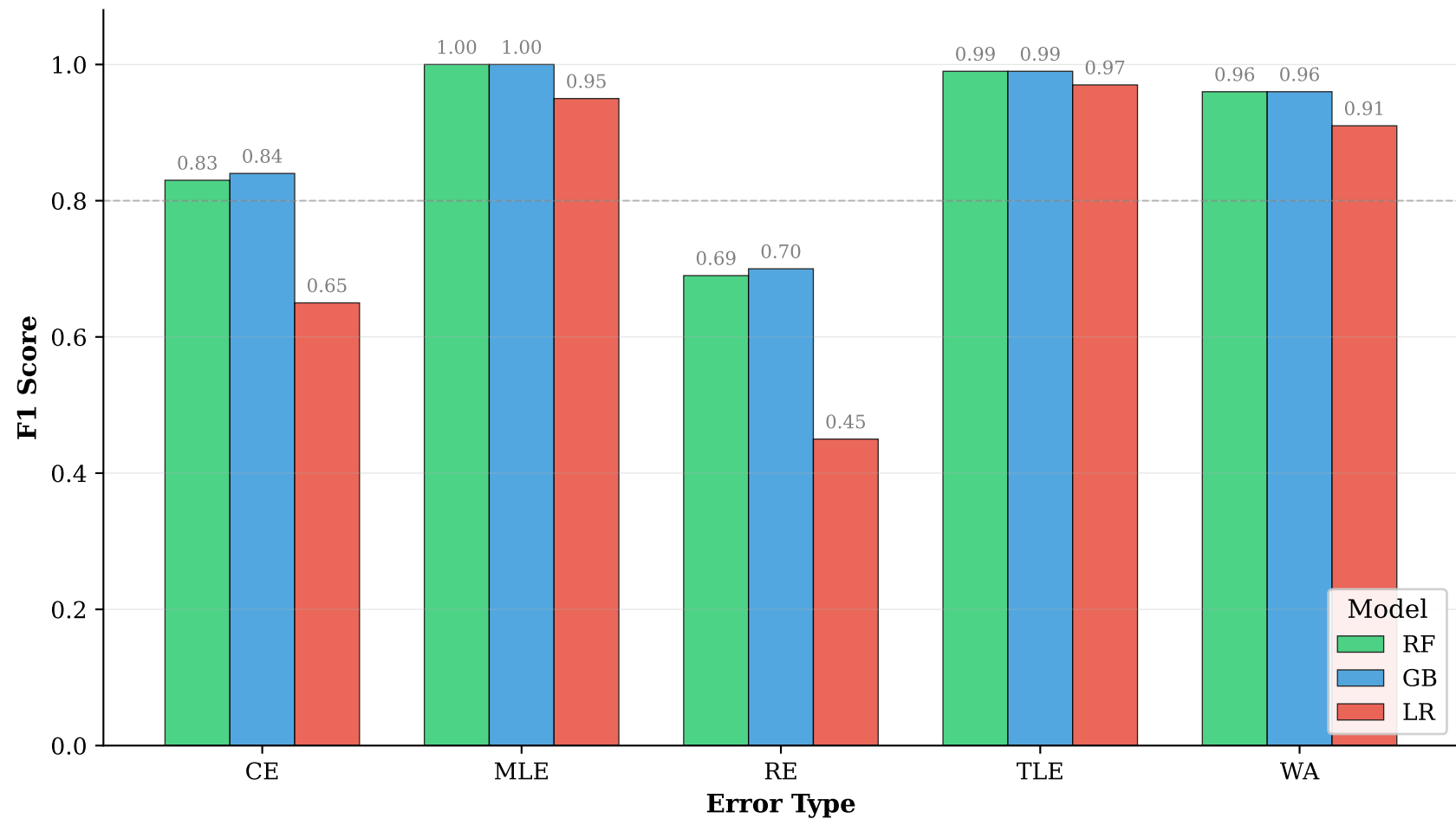
Per-class F1 Score Comparison Across Models
