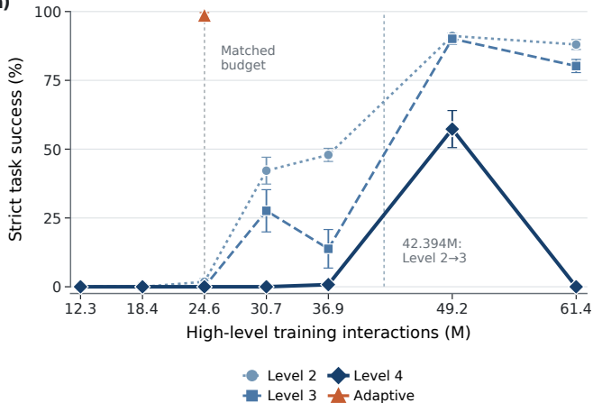
Capability across training budget
