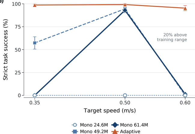
Held out Stage 4 across speed
