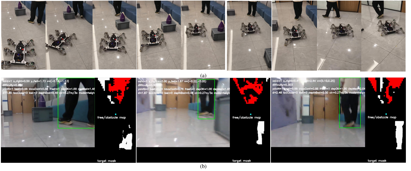
Fig. 7. Real-robot deployment views. (a) The hexapod follows the walking target while sidestepping around staggered corridor obstacles. (b) Three representative onboard times (frames 1, 3, and 5) show the target state and local occupancy-free-space map derived from stereo depth and used by Adaptive.
