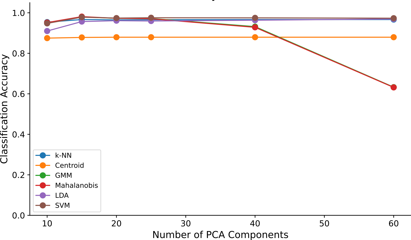
Classifier Accuracy vs PCA Dimensions
