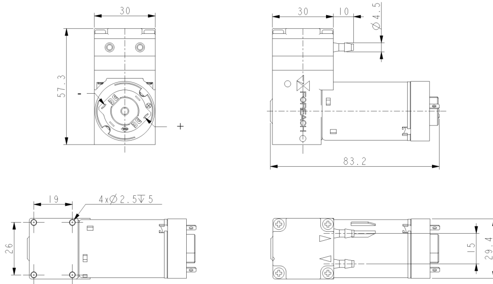
Figure 1 DPL30-24(12)DB - EP/PS Outline Dimensions
