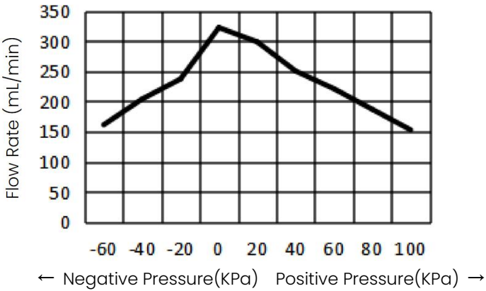
Figure 3 Flow Rate - Pressure Curve
