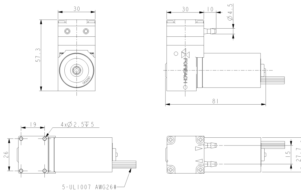
Figure 2 DPL30-24(12)BB - EP/PS Outline Dimensions
