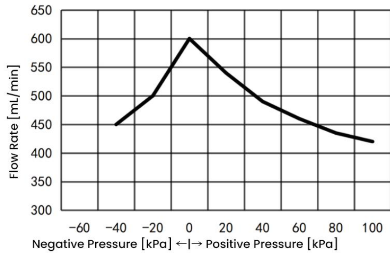
Figure 3 Flow Rate - Pressure Curve
