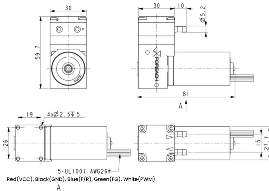
Figure 2 DPL60-24 (12) BB-EP/PS Outline Dimensions
