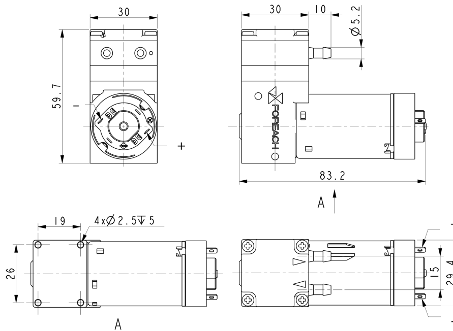
Figure 1 DPL60-24(12)DB-EP/PS Outline Dimensions
