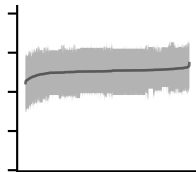
SOX9 risk
