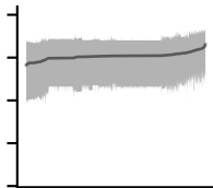
FBXW7 risk
