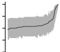
KMT2D risk
