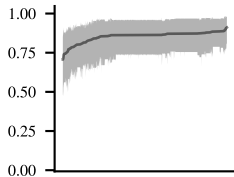
RNF43 risk
