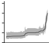
BRAF risk
