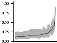
RNF43 risk
