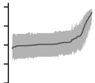
PTPRS risk
