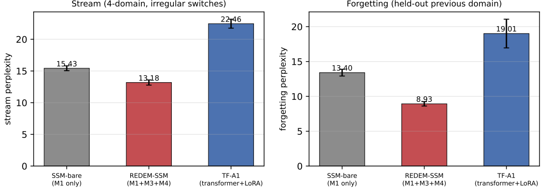
FIG. 3. P4 (10 seeds, four-domain irregular-switch protocol): the full REDEM-SSM stack beats the bare host and the Transformer+LoRA reference on both stream and forgetting perplexity (paired, 10/10).
