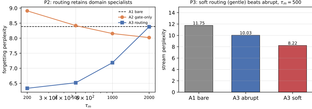
FIG. 2. Left (P2): forgetting perplexity vs. \tau_m — routing (A3) retains domain specialists below the bare baseline (A1, dashed); gating-only (A2) does not. Right (P3): soft routing beats abrupt on stream perplexity at \tau_m=500 (“gentle wins”).
