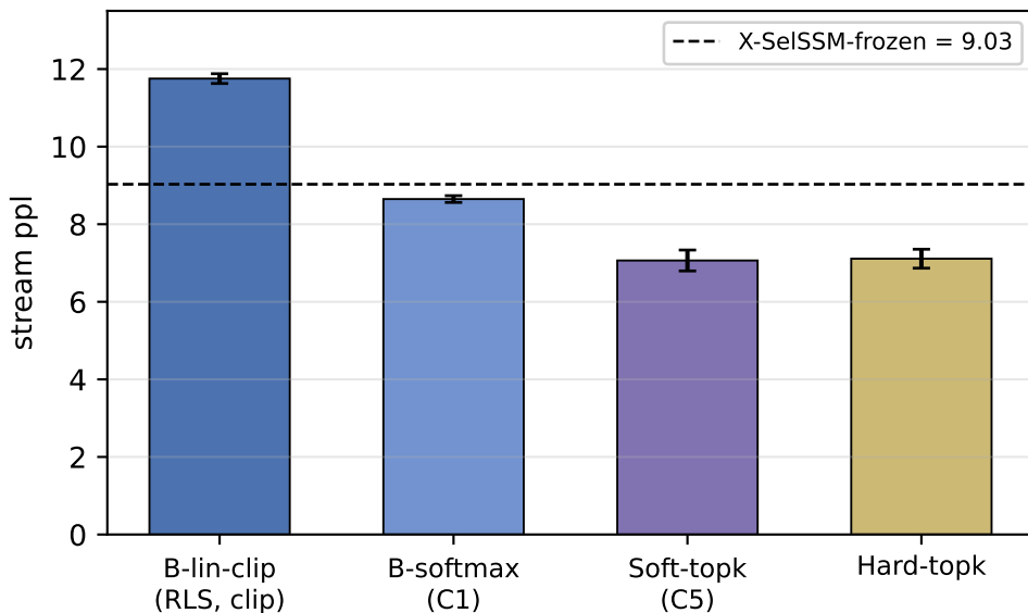
Stream perplexity (10 seeds, mean \pm std)
