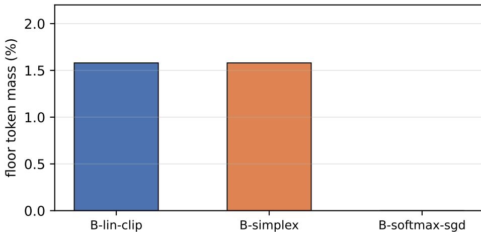
Range fixes relocate the artifact; the objective removes it (C2 vs C1)
