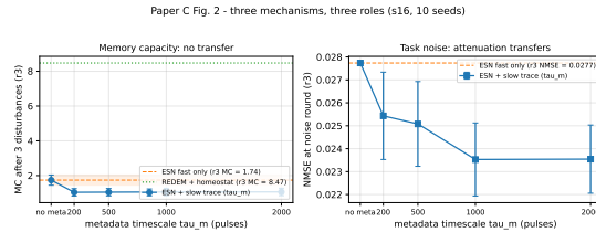
Figure 2: Post-disturbance recovery vs. metadata timescale (Paper C, Fig. 2; s16, 10 seeds). Left: r_3 MC — esn-dual stays 0.68–0.70 below esn-fast at every \tau_m , while the homeostat-regulated substrate (redem-reg, no metadata) sits at 8.47. Right: r_3 NMSE — the readout-noise attenuation transfers at every \tau_m .
