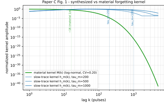
Figure 1: Synthesized vs. material forgetting kernel (Paper C, Fig. 1): the slow-trace kernel h_m (Eq. 2, \tau_m = 200/500/1000 pulses) has a zero at zero lag, a finite peak lag, and an exponential tail with 1/e horizon exactly \tau_m ; the material kernel M (Paper A, log-normal, CV 0.20) is fixed by physics ( 1/e \sim 16 pulses).
