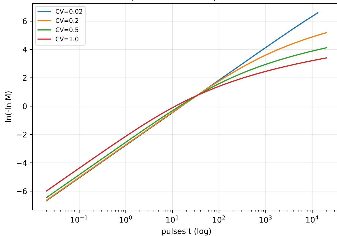
(c) Weibull plot: stretched-exp would be linear
