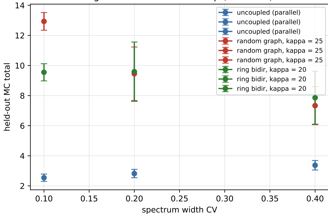
Fig. S1: task-level CV sweep (10 seeds)
