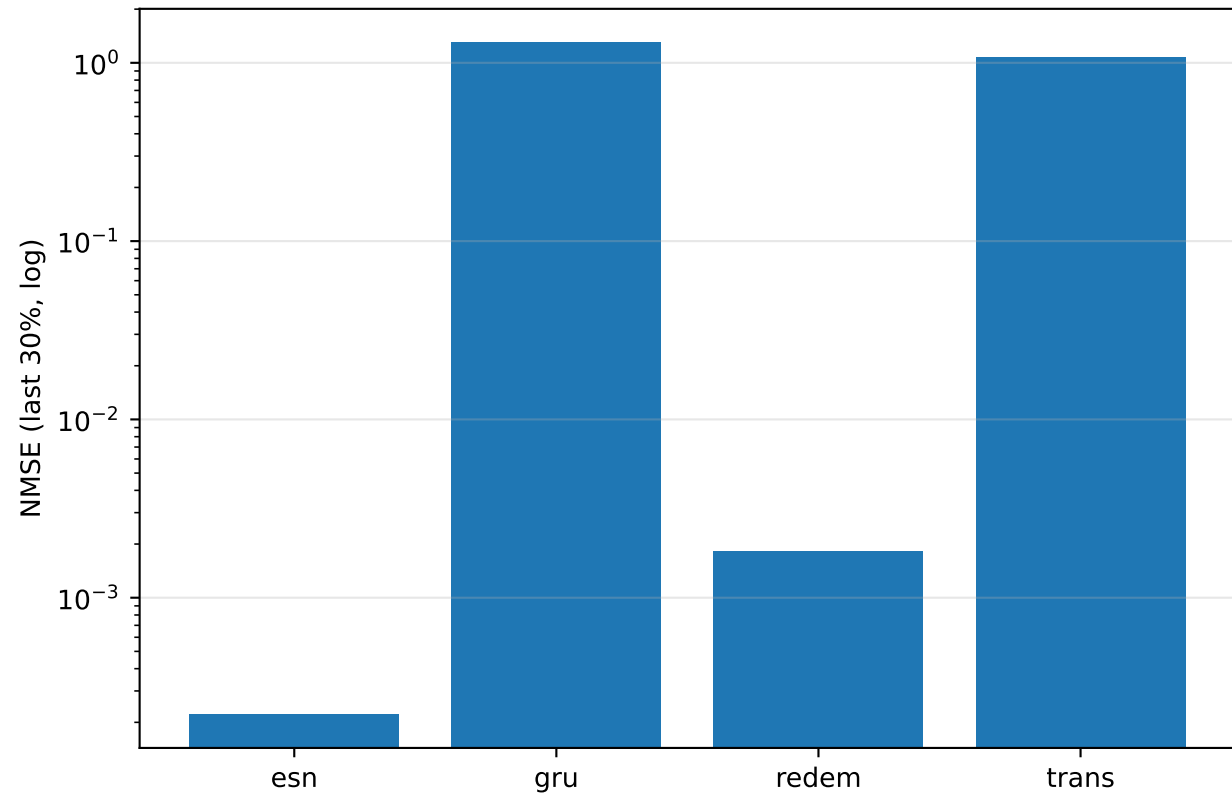
S9: Mackey-Glass forecasting
