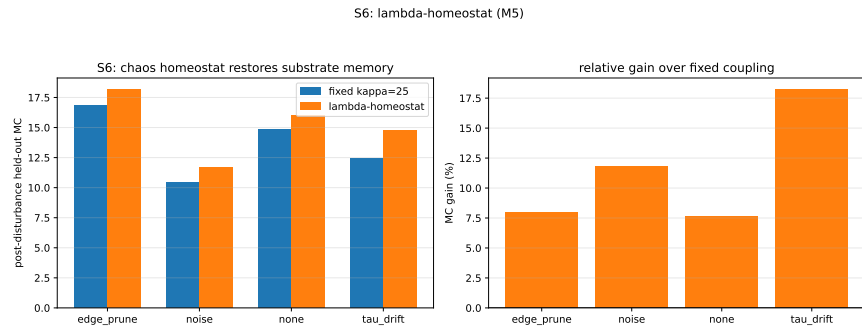
Figure 4: Chaos homeostat robustness (Paper B, Fig. 4): post-disturbance held-out memory gains over fixed coupling.
