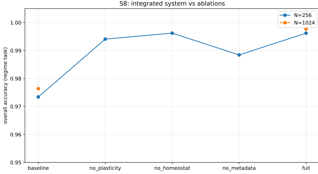
Figure 5: Ablation matrix on regime_switch (Paper B, Fig. 5): full system vs. single-mechanism removals and the bare baseline.
