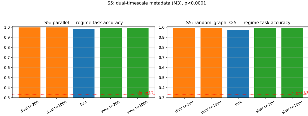
Figure 3: Dual-timescale metadata on regime_switch (Paper B, Fig. 3): fast vs. dual vs. slow readouts, accuracy and adaptation time.
