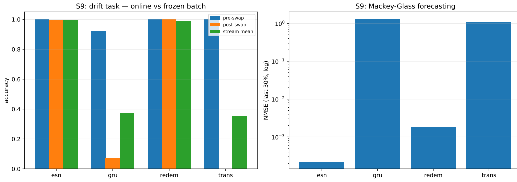
Figure 6: Baseline showdown (Paper B, Fig. 6): REDEM, matched online ESN, and frozen GRU / tiny transformer on drift_binary and Mackey-Glass.
