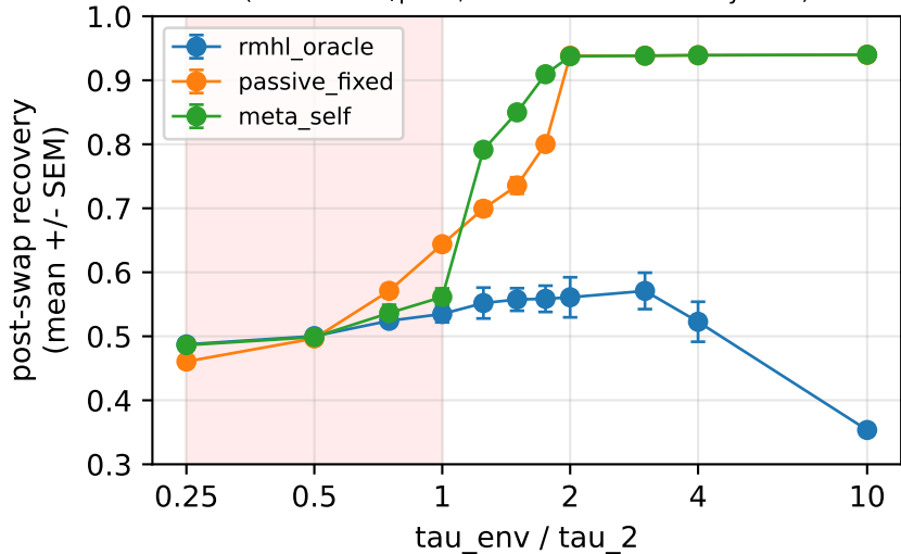
S58e: D2 threshold in the interior points of the sweep (n=10 seeds/point; threshold bracketed by data)
