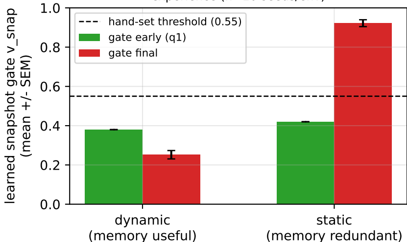
S59 (G1): the memory layer learns WHEN to keep experience (n=10 seeds/env)
