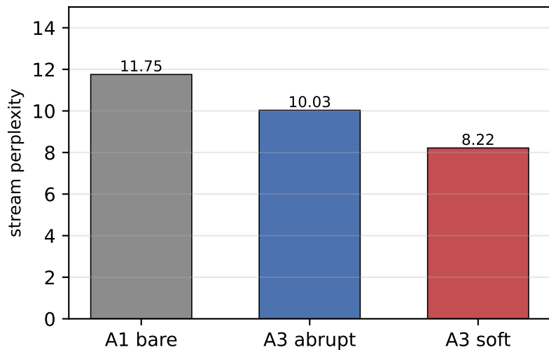
P3: soft routing (gentle) beats abrupt, \tau_m = 500
