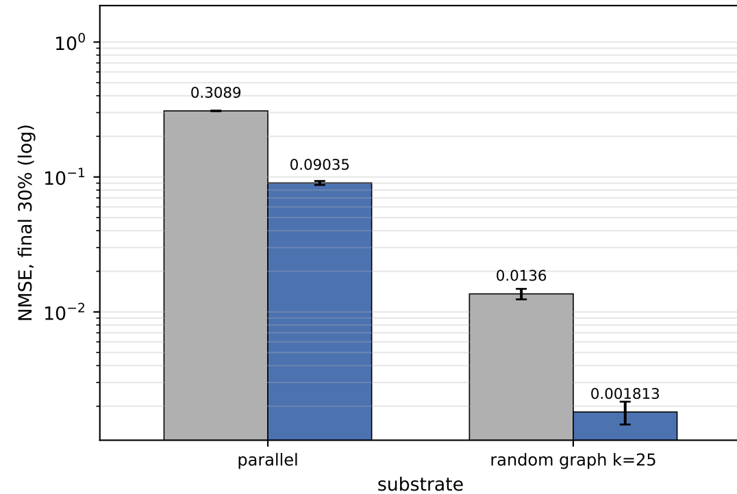
(c) mackey_glass: final-30% NMSE (10 seeds)
