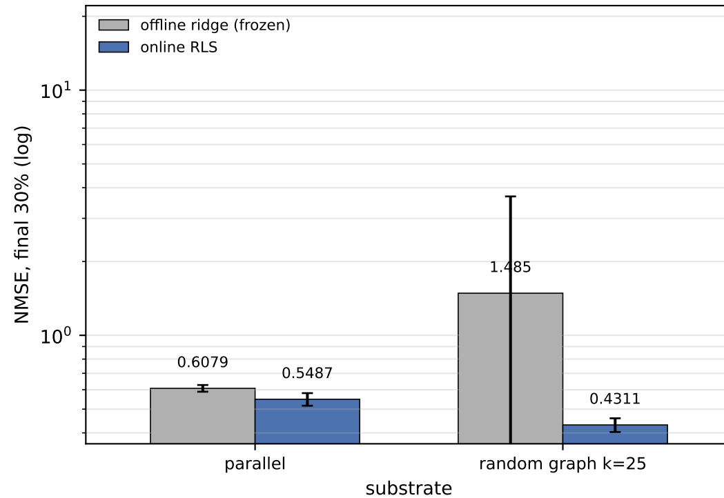
(b) narma10: final-30% NMSE (10 seeds)
