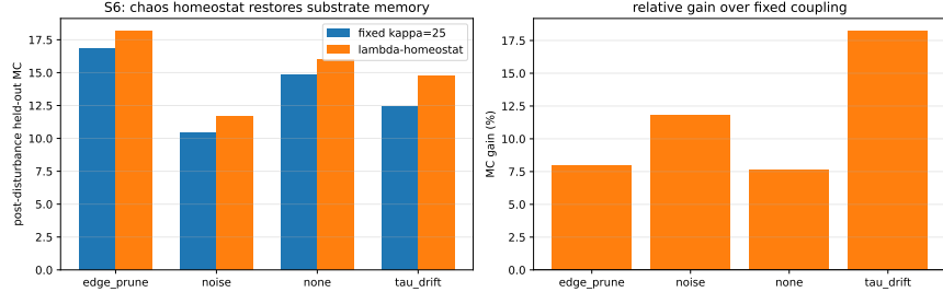
Figure 4: Chaos homeostat robustness: post-disturbance held-out memory gains over fixed coupling (reproduced from companion Paper A [11]).
