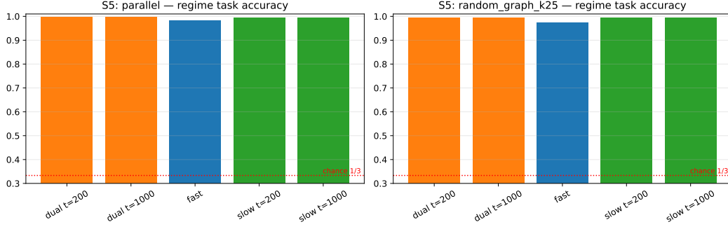
Figure 3: Dual-timescale metadata on regime_switch: fast vs. dual vs. slow readouts, accuracy and adaptation time.
