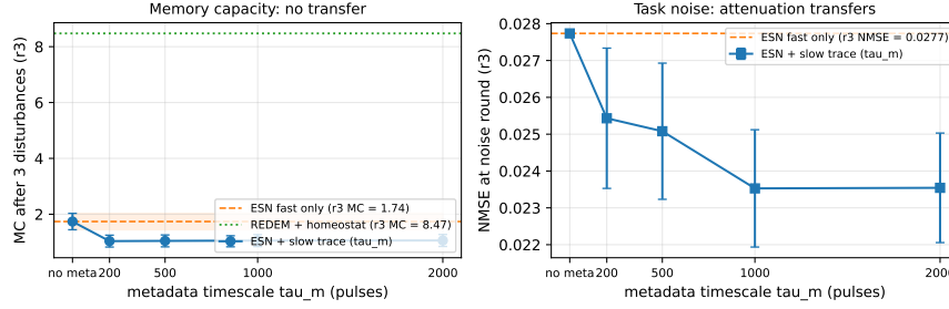
Figure 2: Post-disturbance recovery vs. metadata timescale (10 seeds). Left: r_3 MC — esn-dual stays 0.68–0.70 below esn-fast at every tested \tau_m , while the homeostat-regulated substrate (redem-reg, no metadata) sits at 8.47. Right: r_3 NMSE — the readout-noise attenuation transfers at every tested \tau_m .
